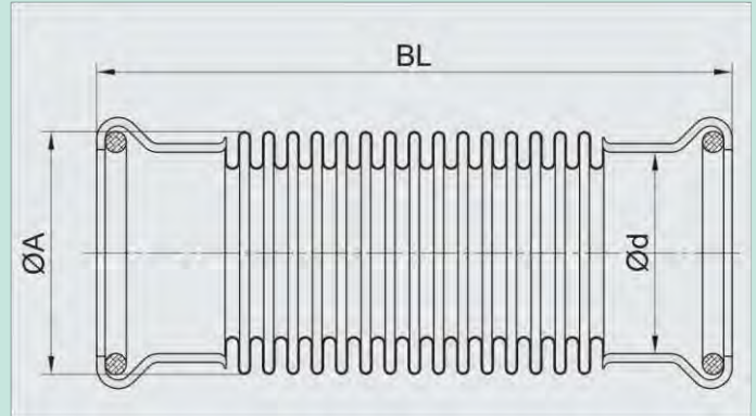
This expansion joint is not suitable for vibrations.
